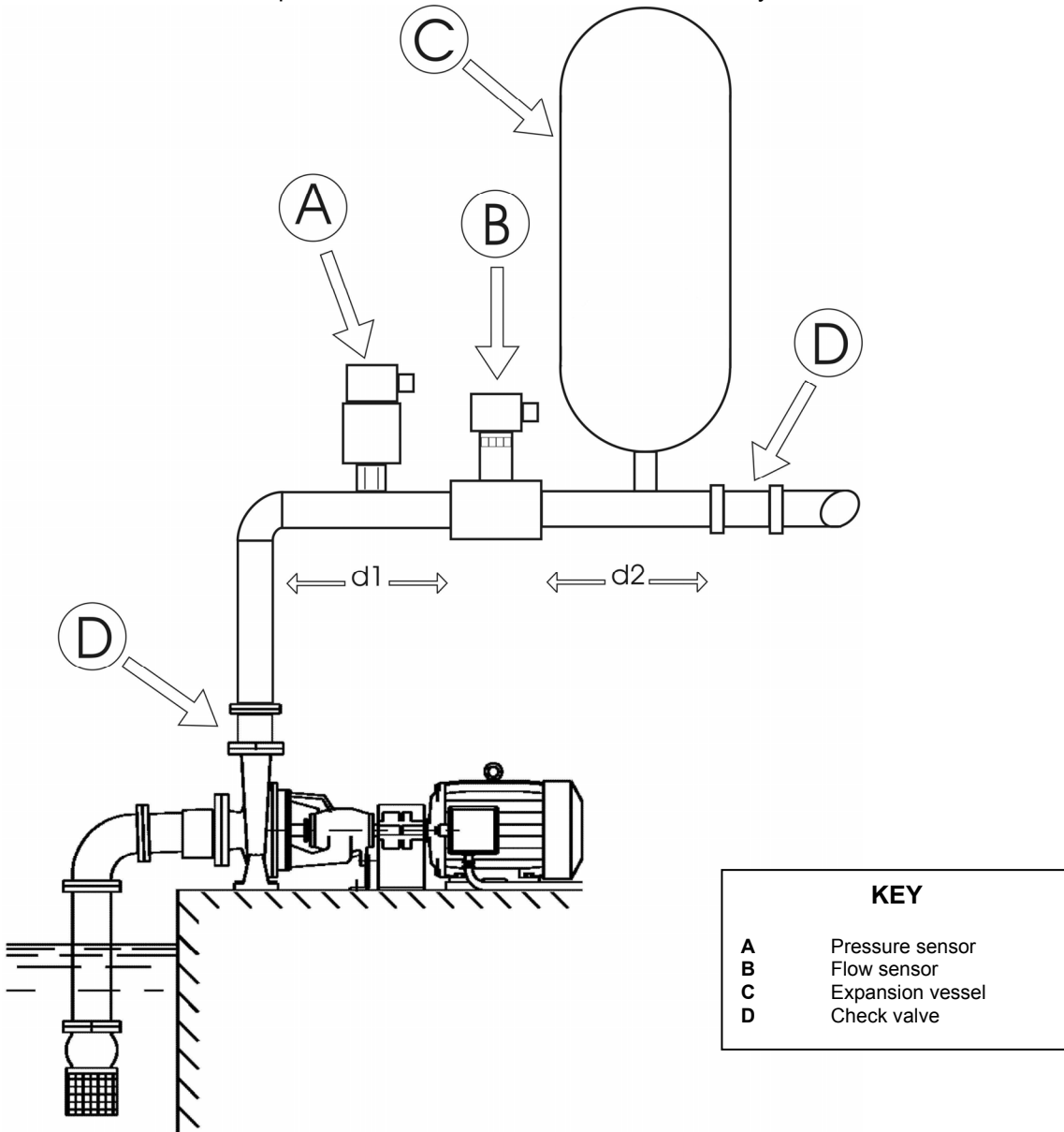
Figure 8: Hydraulic installation
