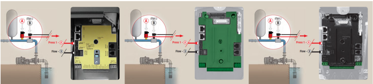
Figure 9: Sensor connections
