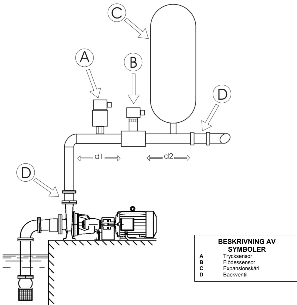
Fig. 8: Hydraulisk installation
