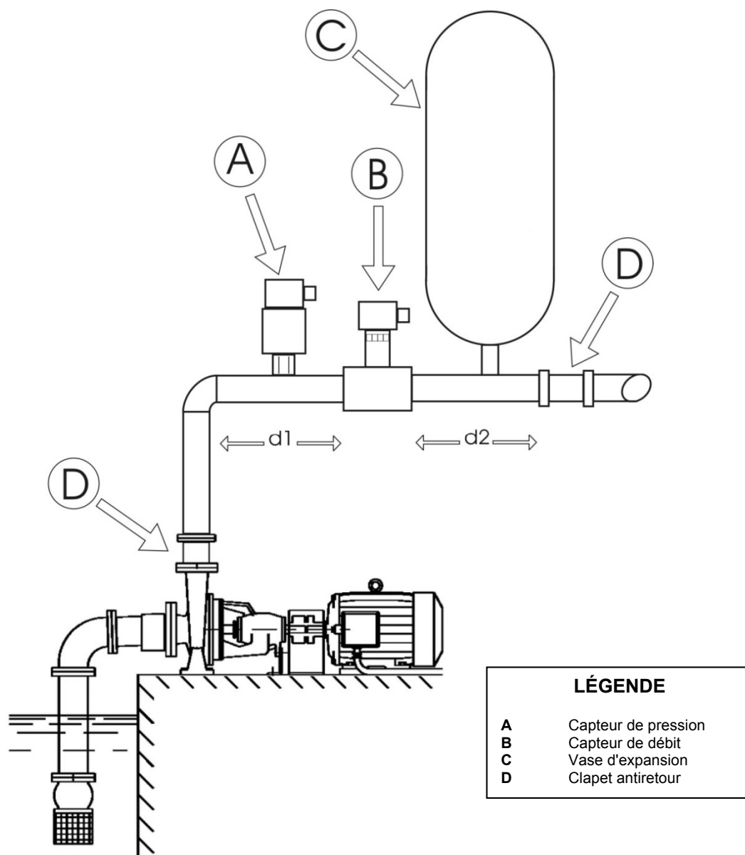
Figure 8: Installation hydraulique
