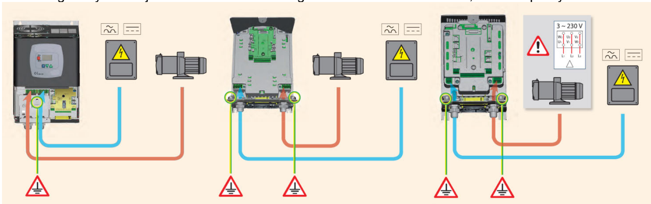
Figure 6: Electrical connections
