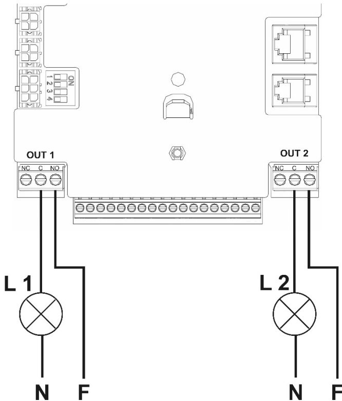
Figure 11: Example of output connections
