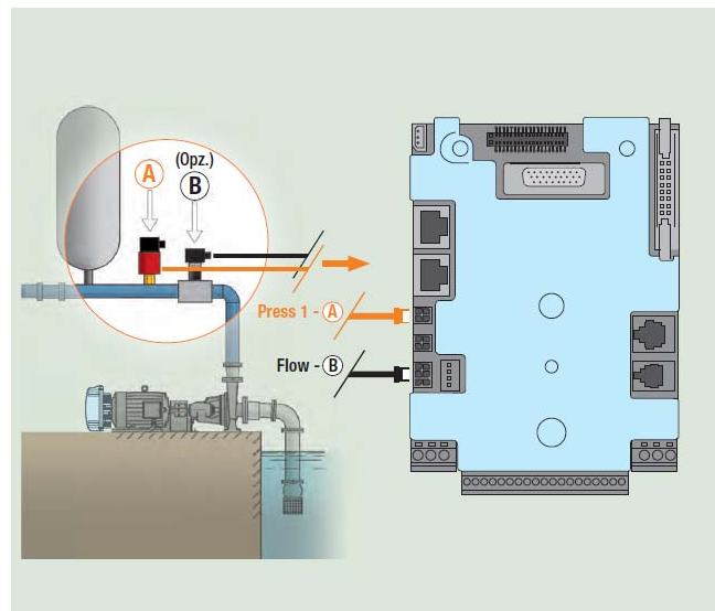
Figure 8: Sensor connections
