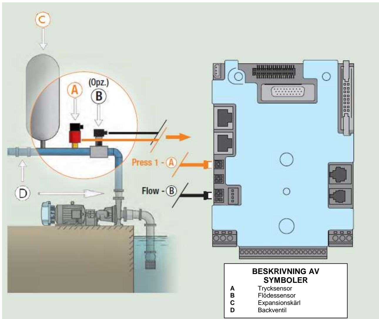
Fig. 7: Hydraulisk installation
