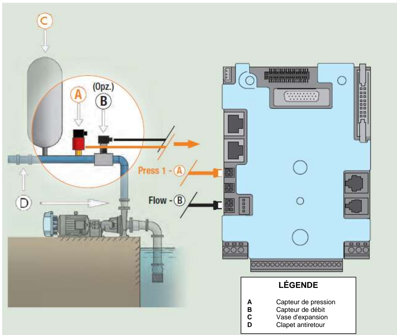
Figure 7: Installation hydraulique
