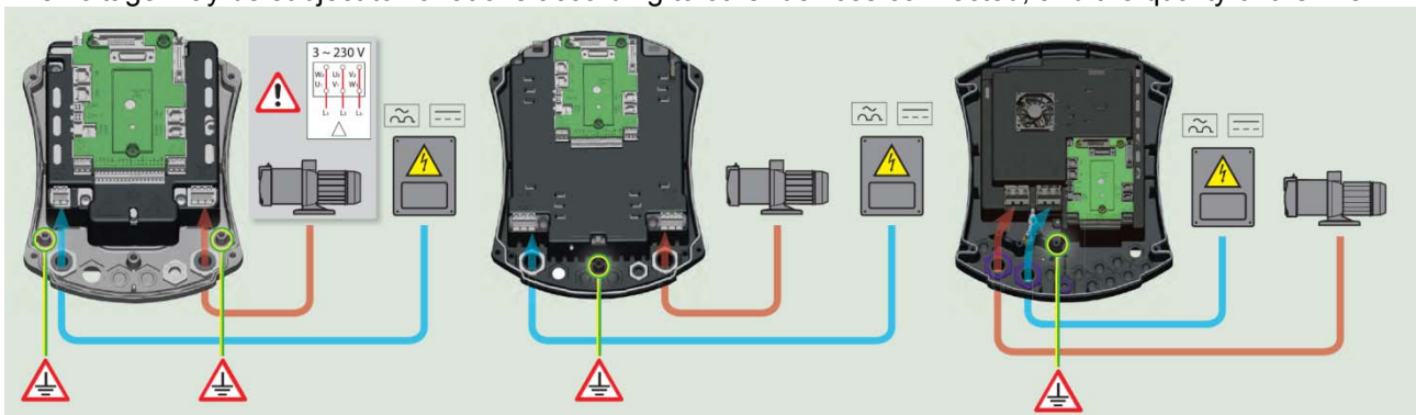
Figure 5: Electrical connections
